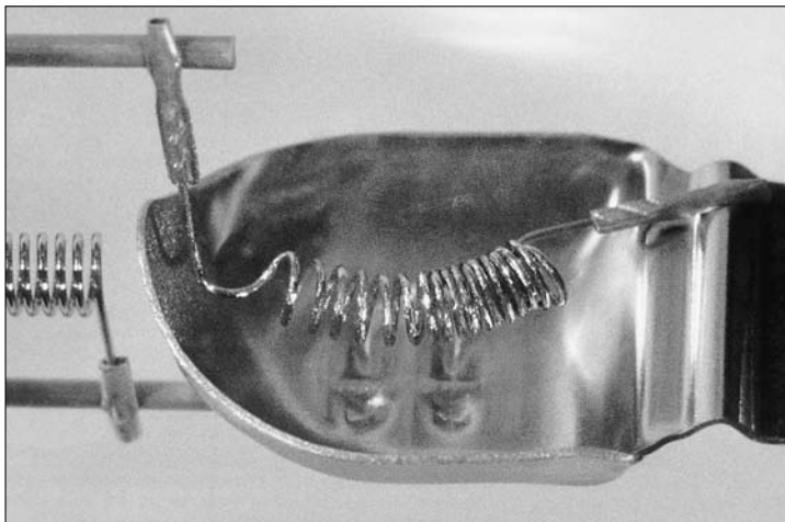
Reflector bulb of a motorcycle after a collision with a pedestrian
